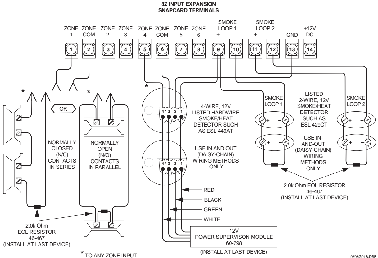
Figure 4. Typical Card Wiring
